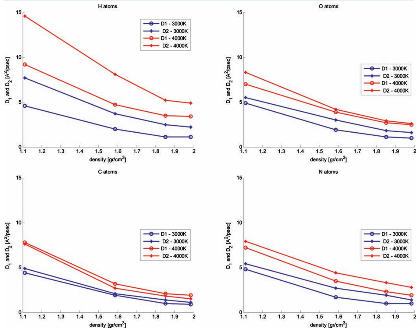
Figure 24. Diffusion coefficients in the time region [t_0, t_b] ( D_1 ) and [t_b, t_{\text{end}}] ( D_2 ), as a function of density, for hydrogen, oxygen, carbon, and nitrogen atoms.
