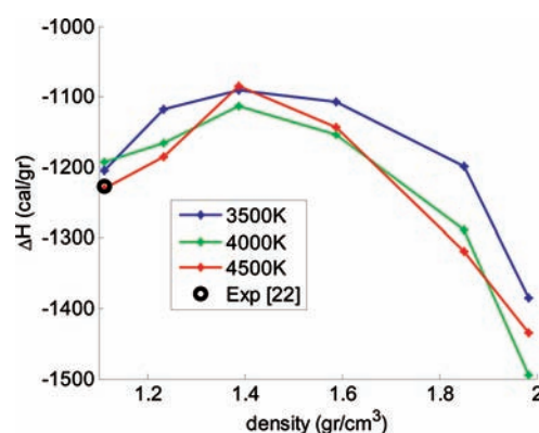
Figure 19. NM decomposition enthalpy change versus density for various temperatures. Also marked is the measured heat release in NM detonation 22 (plotted at ambient density).
