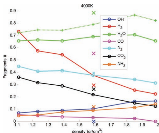
Figure 17. Calculated stable fragments fraction as a function of NM density at 4000 K (○, solid lines). Crosses represent measured detonation products 22 (plotted at CJ density). Also shown is the sum of H 2 O and OH fragments (+, dotted line).
